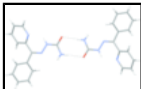
Fig. 2. Centrosymmetric dimers linking two molecules of H2Bz4PS in the crystal packing. The dotted lines represent the hydrogen bonds of the type N—H...O.
