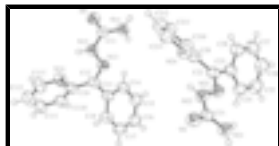
Fig. 1. The molecular structure of the title. Displacement ellipsoids are drawn at the 50% probability level.
